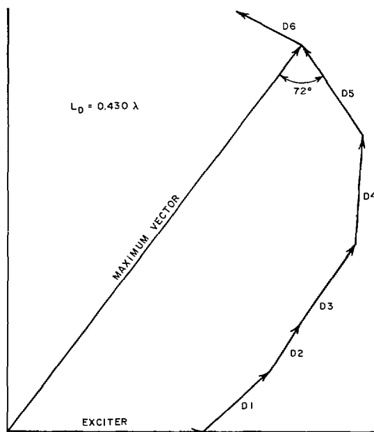
Fig. 14. Phase velocity diagram for 8-element array with L_D = 0.430\lambda .
