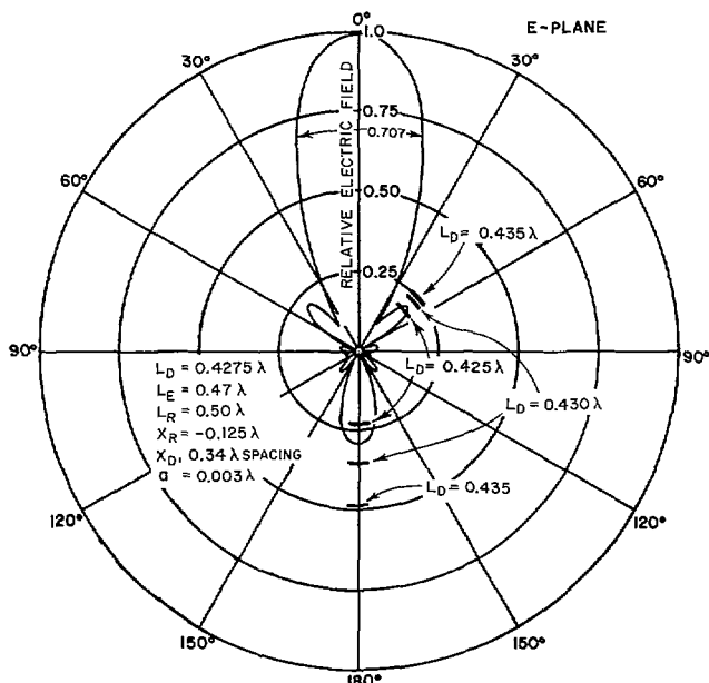
Fig. 15. E -plane pattern of optimum 8-element array with side lobe levels indicated for several other versions of array.
