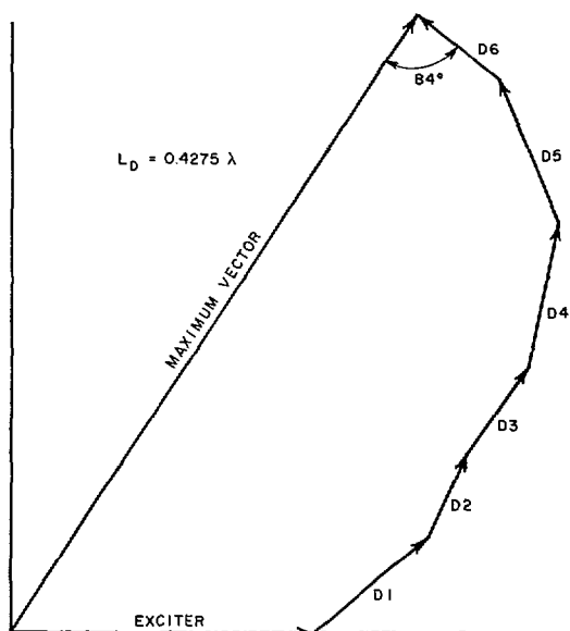
Fig. 13. Phase velocity diagram for 8-element array with L_D = 0.4275\lambda .
