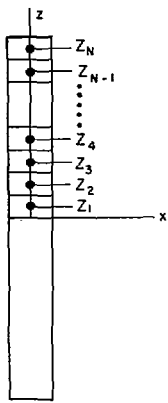
Fig. 3. Parasitic element with N matching points along its axis.
