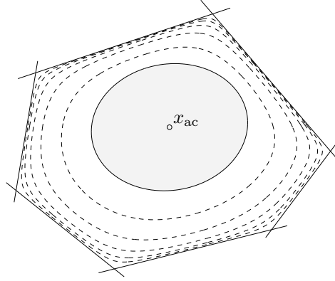
Figure 8.7 The dashed lines show five level curves of the logarithmic barrier function for the inequalities defining the polyhedron C in figure 8.5. The minimizer of the logarithmic barrier function, labeled x_{ac} , is the analytic center of the inequalities. The inner ellipsoid \mathcal{E}_{\text{inner}} = \{x \mid (x - x_{ac})^T H(x - x_{ac}) \leq 1\} , where H is the Hessian of the logarithmic barrier function at x_{ac} , is shaded.
