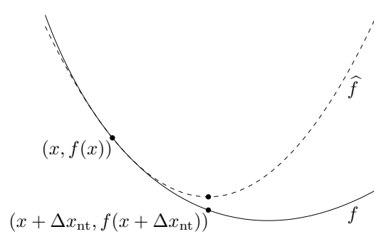
Figure 9.16 The function f (shown solid) and its second-order approximation \hat{f} at x (dashed). The Newton step \Delta x_{\text{nt}} is what must be added to x to give the minimizer of f .
