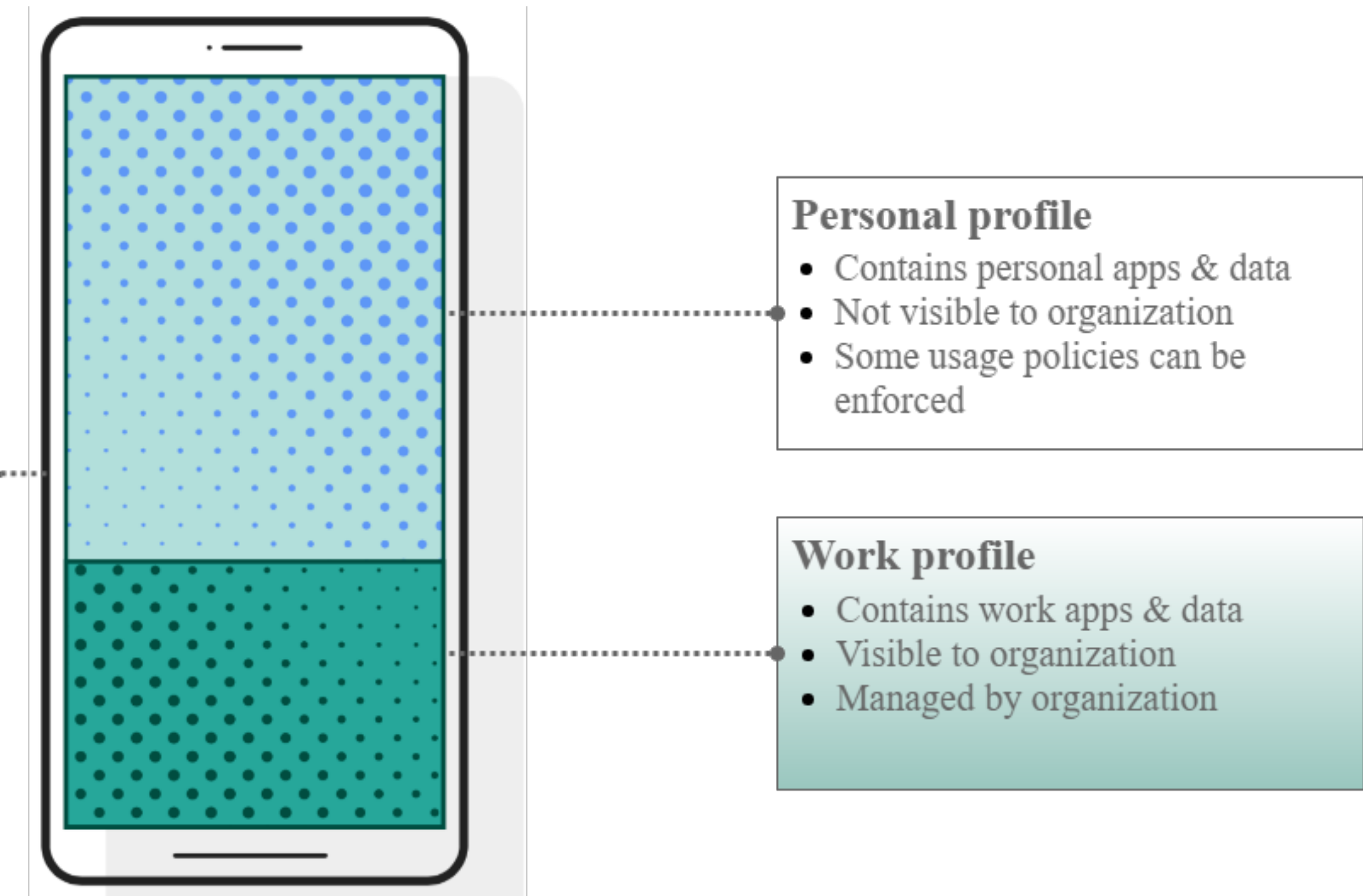
Work profile for mixed-used company-owned devices
